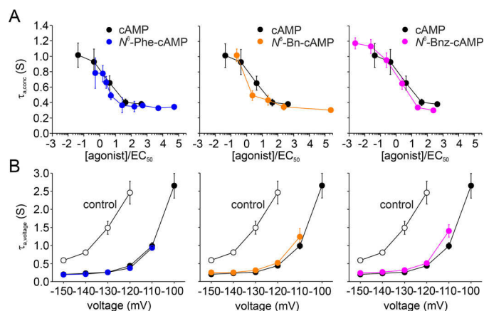
Figure 4. Activation kinetics for the tested cAMP derivatives. A, activation kinetics in dependence on agonist concentration at a given command voltage of -130 mV. \tau_{a,\text{conc}} values, obtained from approximating a monoexponential equation (Equation 3) to the current time courses, are plotted against the cAMP concentration. Mean values were obtained from three to nine recordings. Black symbols in each plot illustrate the case for cAMP. The protocol used is shown in Fig. 1A. B, activation kinetics in dependence on command voltage at a saturating agonist concentration. \tau_{a,\text{voltage}} values were plotted against the command voltage. Open symbols represent recordings in the absence of ligands and filled symbols in the presence of saturating agonist concentrations. Mean values were obtained from three to 19 recordings. The protocol used is shown in Fig. 1B.
